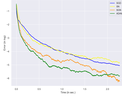
(a) J = 100 - n_{\max} = 19828 (SGD), 4321(SN), (b) J = 200 - n_{\max} = 20000 (SGD), 1983(SN), 9783(SGN), 20000(ADAM) 5433(SGN), 19163(ADAM)
