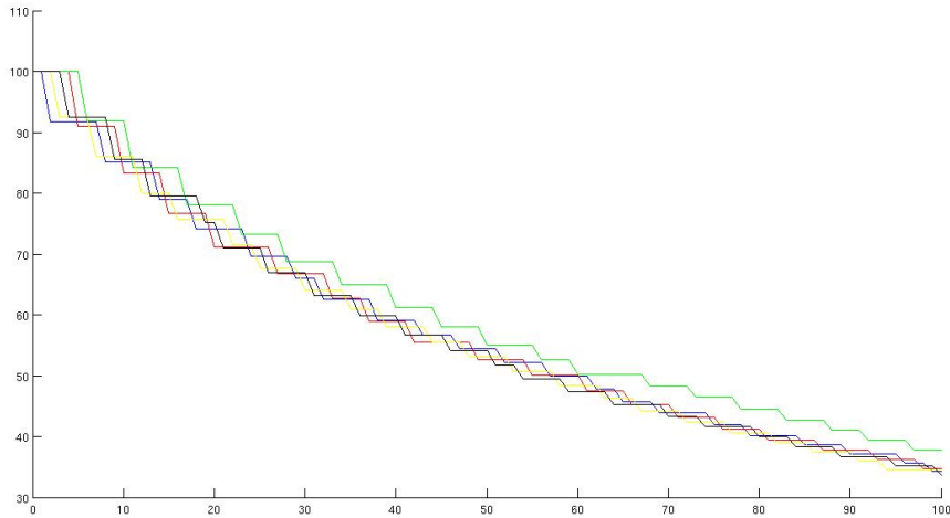
Figure 1: First dataset (p, m, S) = (250, 5, 50) : Norm of each coordinate of residuals along the first 100 iterations of the Boost-Boost \mathcal{D} -Correlation sum algorithm; the sample size n is set to 100.
