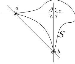
FIGURE 6.1. The foliation of \mathbb{P}_{\mathbb{C}}^2 given by \omega = d(x^p z^{q-p}/y^q)
