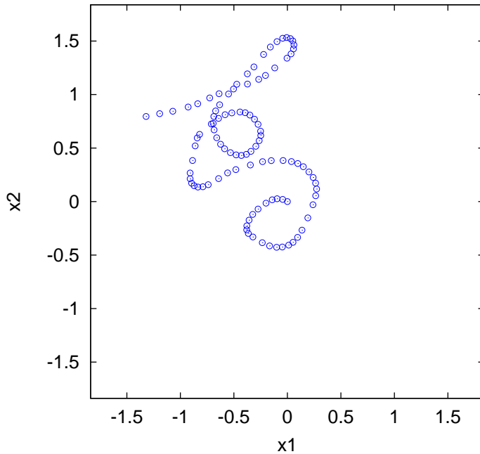
Figure 1: An example of the trajectory t \mapsto x_t = (x_t^1, x_t^2) of the PTWM where the speed of the fish decreases with higher curvature (eq. 2.7). Here \alpha = 1 and c(|\kappa|) = 1/(1 + 2|\kappa|) . The simulation is run during 10 time units, we plot a point each .1 time unit.
